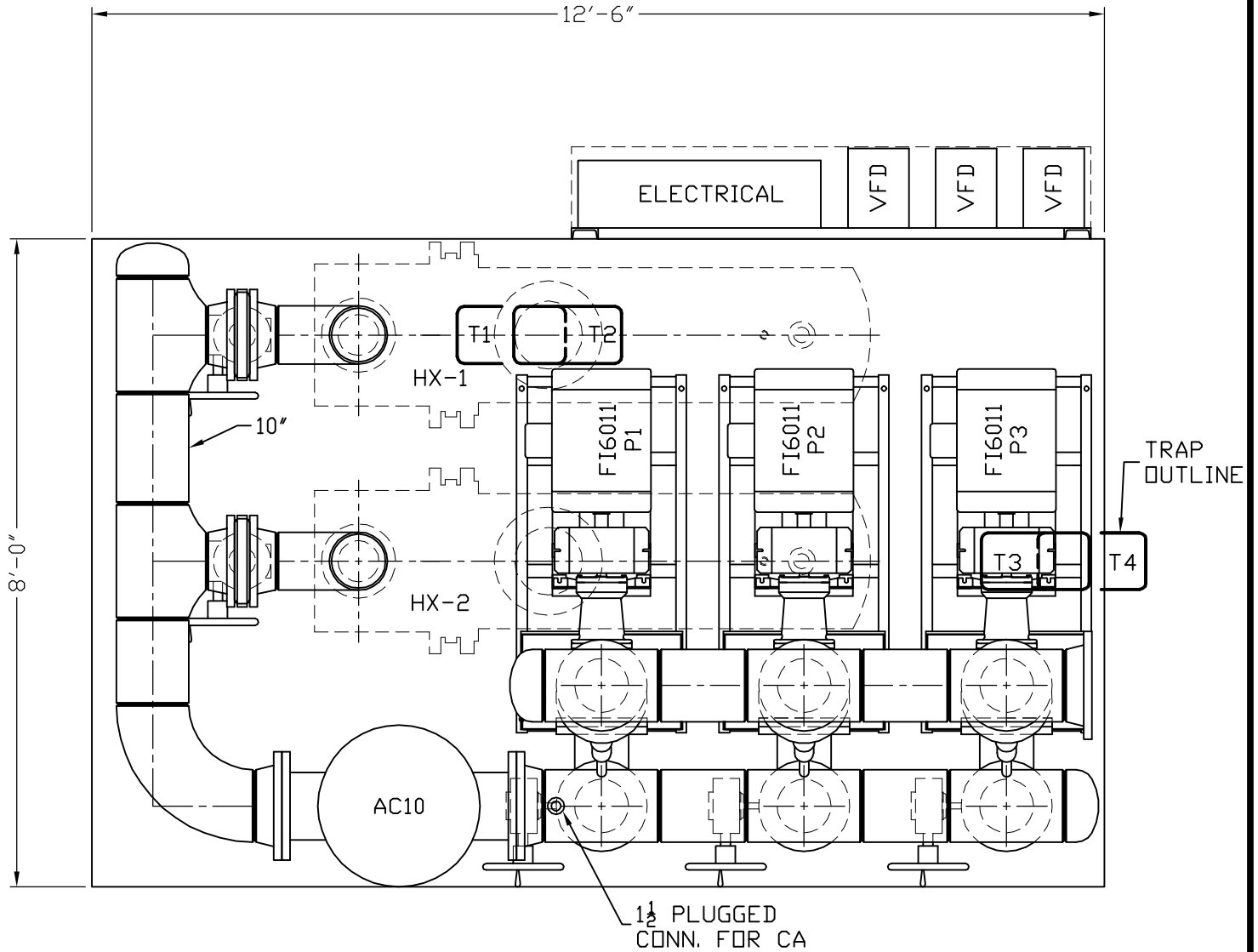
PLAN VIEW
