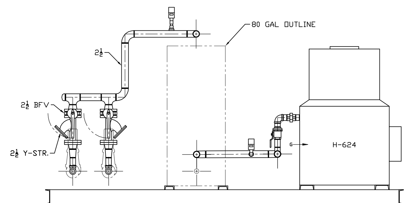
SECTION C-C
