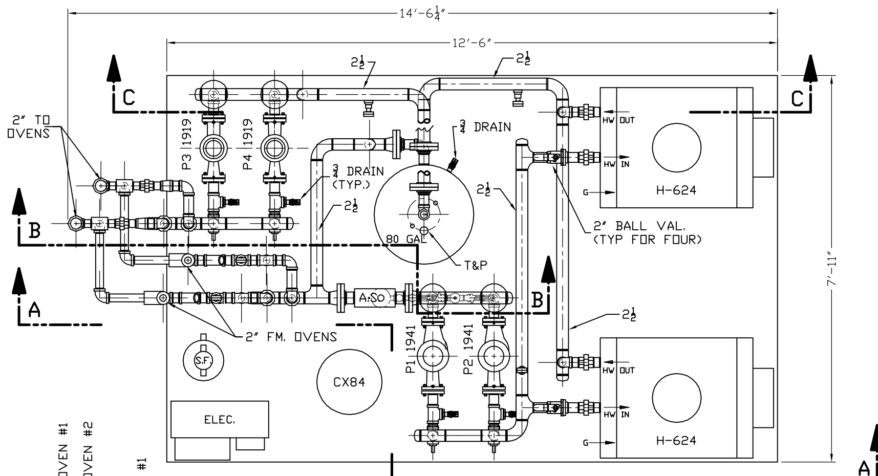
PLAN VIEW
